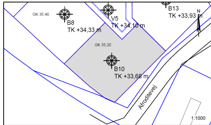
Figur 1 – Situationsplan 1:1000, Parcel nr. 10
